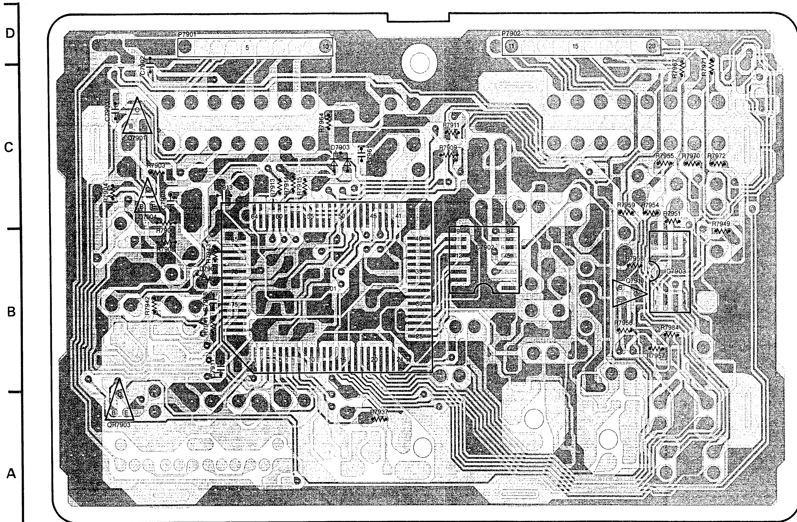
(COMPONENT SIDE)
